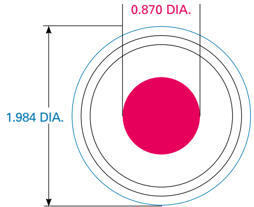
1" LADISH® TC
